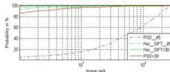
Figure 5. CMC performances for partial prints with rotation distortions.
