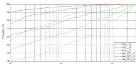
Figure 6. CMC performances for partial prints with rotation and noise distortions.
