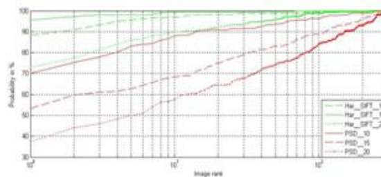
Figure 4. CMC performances for partial prints with noise perturbations
